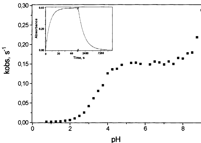
Figure 1. Effect of pH on the first-order rate constant for the hydrolysis of the 2',2',2'-trifluoroethyl monoester of 1,8-naphthalic acid. The inset shows the absorbance at 340 nm as a function of time
